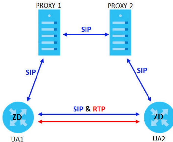
Figure 239 SIP Call Through Proxy Servers
