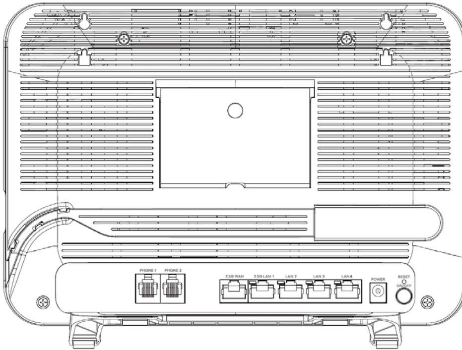
Figure 37 EX5601-T0/EX5601-T1
