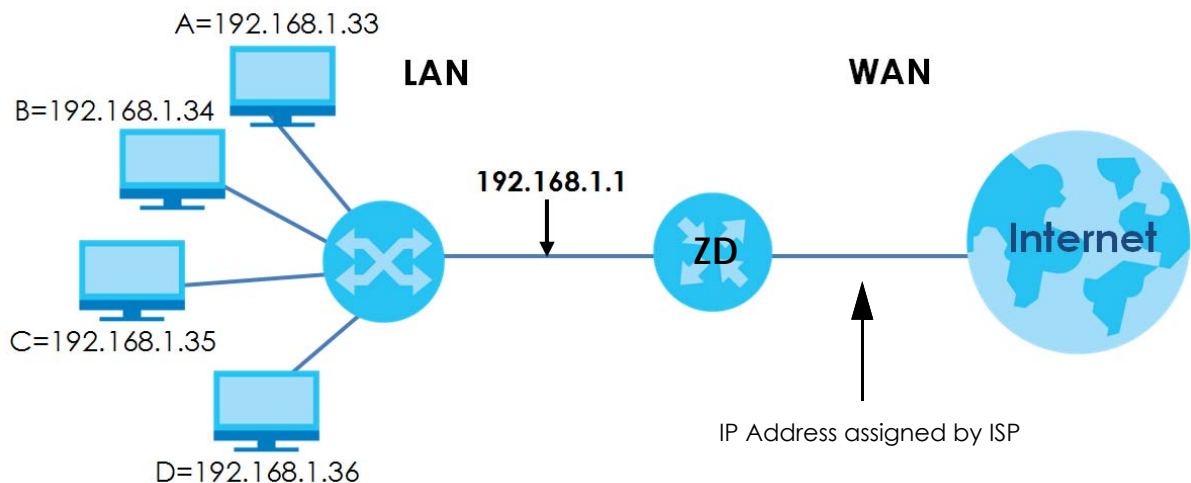
Figure 183 Multiple Servers Behind NAT Example
