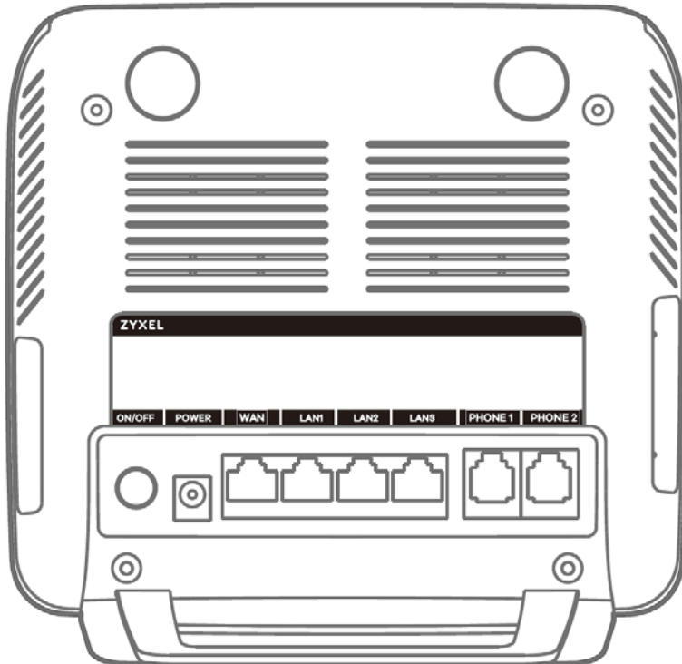
Figure 34 EX3501-T0
