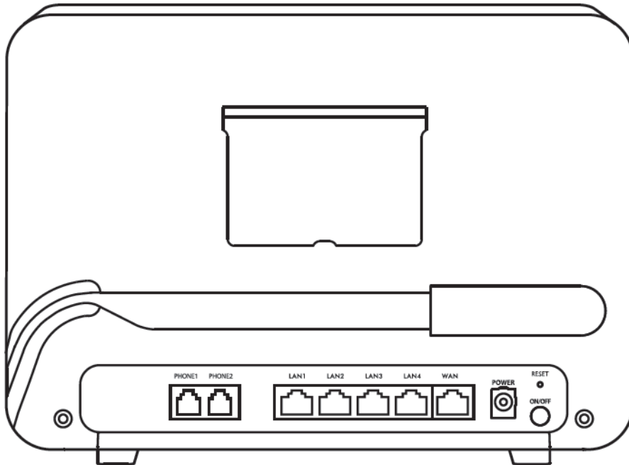
Figure 30 EX5401-B0 / EX5401-B1
