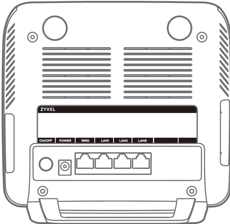
Figure 34 EX3501-T0
