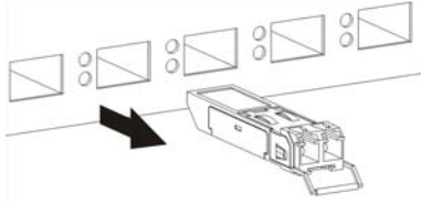
Figure 41 Transceiver Removal Example
