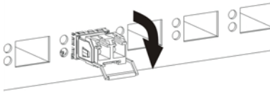
Figure 41 Transceiver Removal Example
